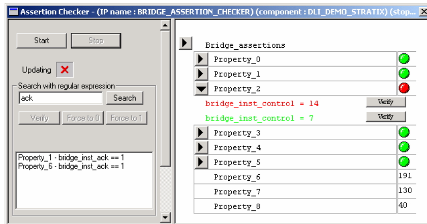
Figure 1: Temento DiaLite tool displaying an assertion failure
